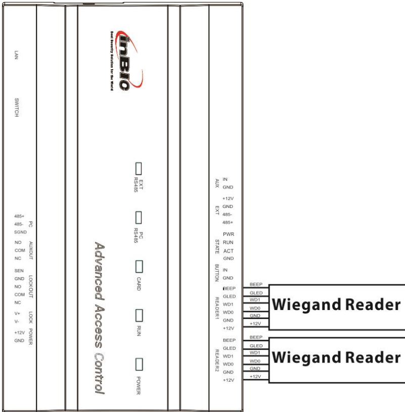
Connection between InBio-160 and Readers
