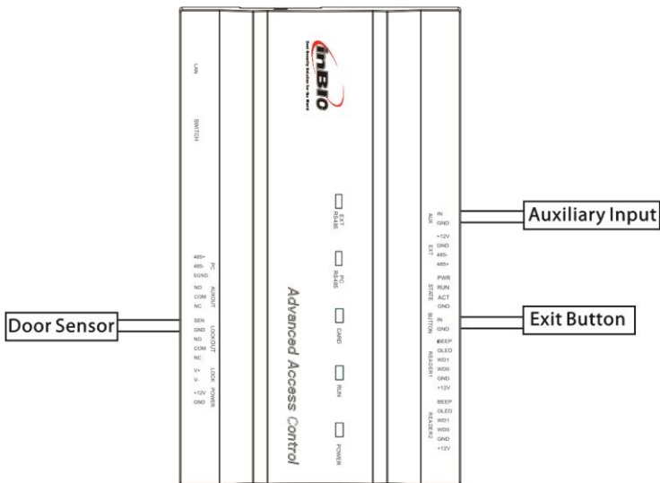
Connections between InBio-160 and external accessories
