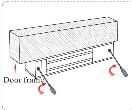
Step 5: Use cross screwdriver to install wire box cover and the anti-dismantle screws.
