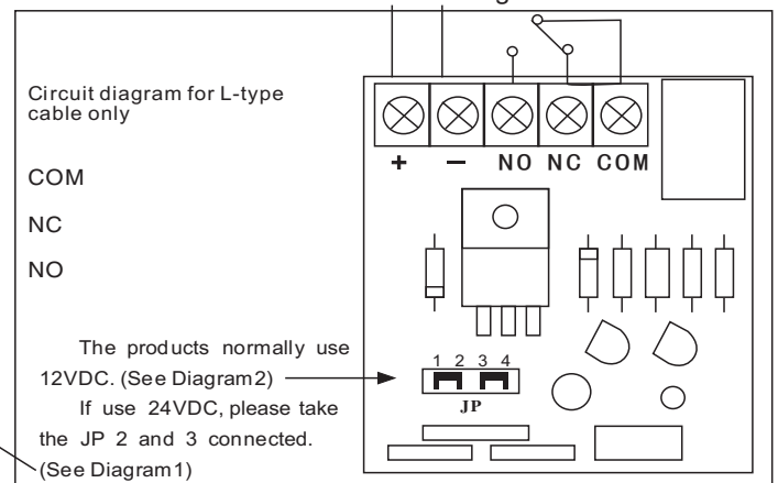
Diagram 1(12VDC)
