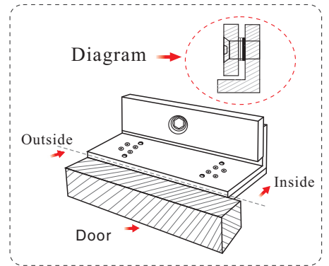
Step 9: Fix Z-bracket to relevant position on the door leaf. (Note: Keep tight contact between the sub-plate and the lock)
