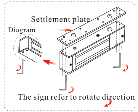
Step 3: Use Allen key to separate the connecting plate from the bottom of the lock. Be careful to hold the screw to prevent slipping.
