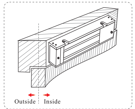
Step 6: Status of the lock after installation
